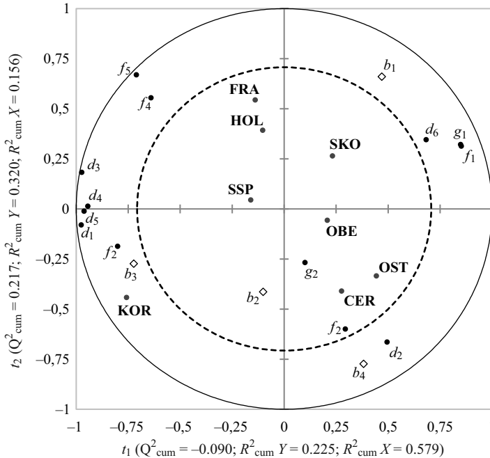
Fig. 2. A circle diagram presented the correlations among spelt cultivars, the quality properties of grain ( g_1, g_2 ), flour ( f_1-f_5 ), dough ( d_1-d_6 ) and bread ( b_1-b_4 ) vs. the first two PLS components of t_1 and t_2 . The dotted circle represented a correlation of 0.7. CER: cv. Ceralio ; SKO: cv. Schwabenkorn ; FRA: cv. Franckenkorn ; HOL: cv. Holstenkorn ; SSP: cv. Schwabenspeltz ; OST: cv. Ostro ; OBE: cv. Oberkulmer Rotkorn ; KOR: cv. Korweta
