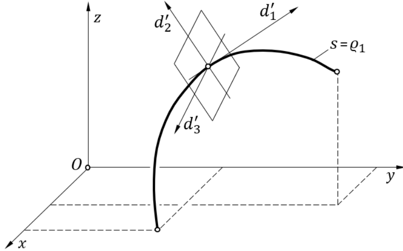
Fig. 1. The Frenet trihedron on the one-dimensional physical line immersed in the Euclidean space.
