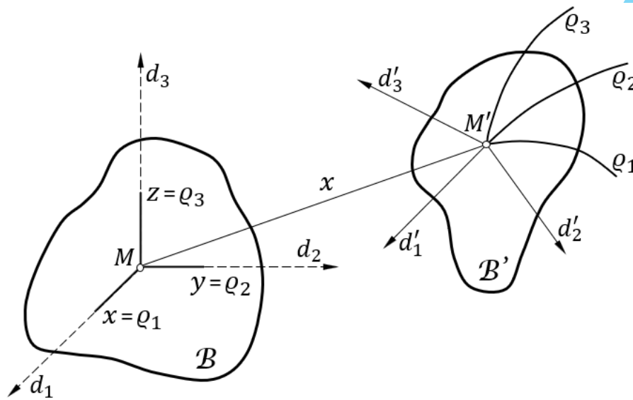
Fig. 2. Cosserats' concept of a moving frame (1896).
