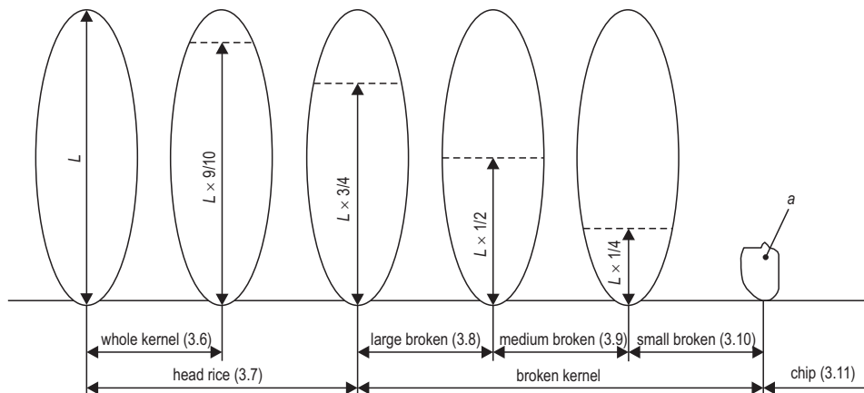
Fig. 1. Grain sizes and fractions of grain parts Source: based on PN-ISO 7301:2004. Ryż – Wymagania (2004).
