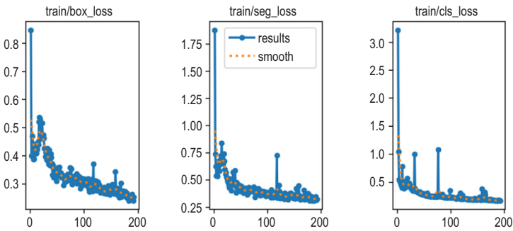
Fig. 6. Loss Value Charts
