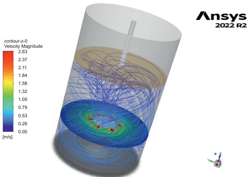
Fig. 11. Velocity distribution at the center of the impeller disk for the MRF+VoF model, 480 rpm, and 1000 iterations
