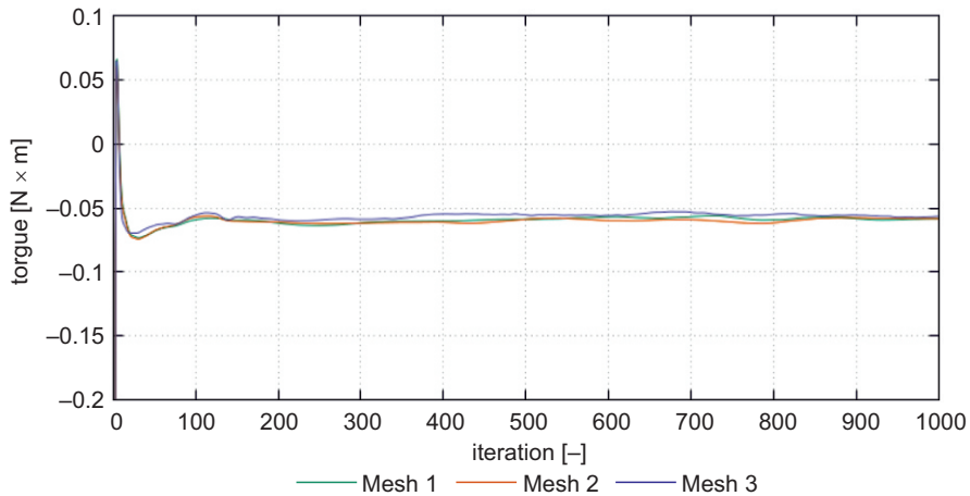
Fig. 7. Torque monitor graph for the MRF model, 480 rpm, and three grid variants
