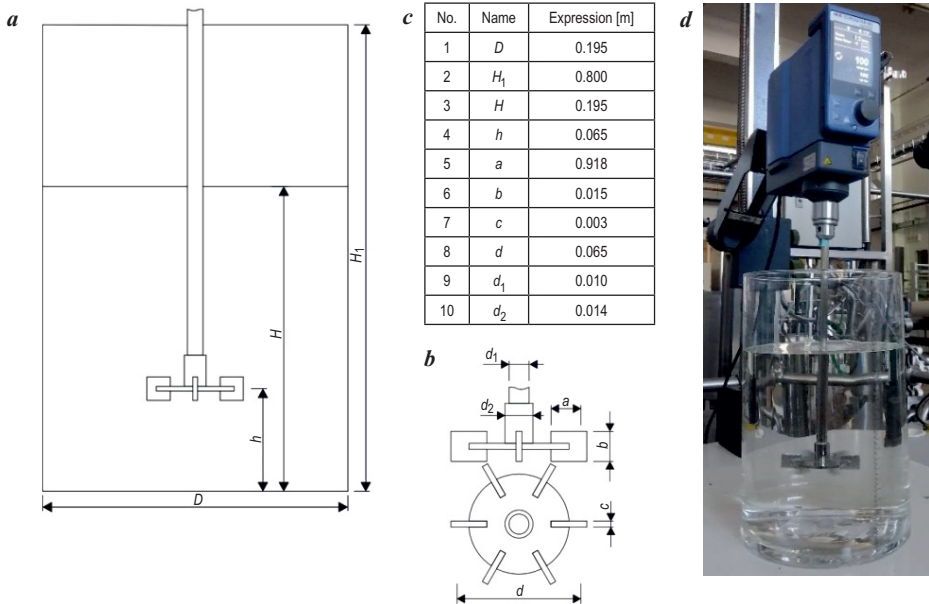
Fig. 1. Laboratory workstation: a) geometry of the tank with the impeller, where H denotes the liquid filling height and H = D (internal tank diameter), and h = H/3 ; b) impeller geometry; c) tank and impeller geometric parameters; d) photograph of the laboratory workstation
