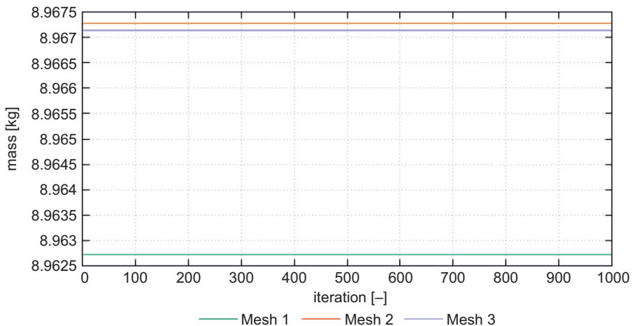
Fig. 8. Mass monitor graph for the MRF model, 480 rpm, and three mesh variants
