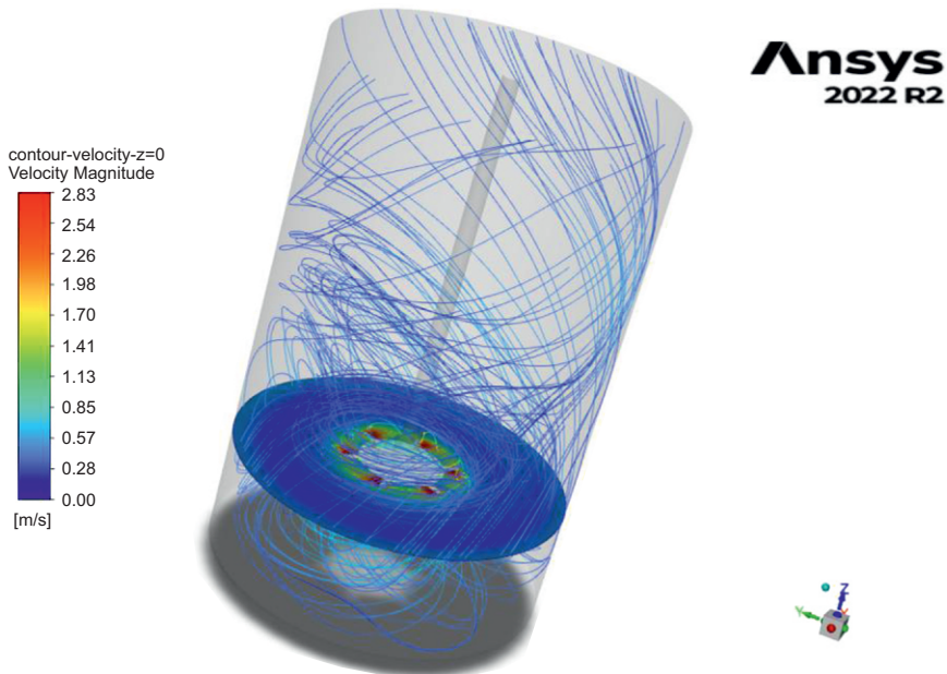
Fig. 10. Velocity distribution at the center of the impeller disk for the MRF model, 480 rpm, and 1000 iterations
