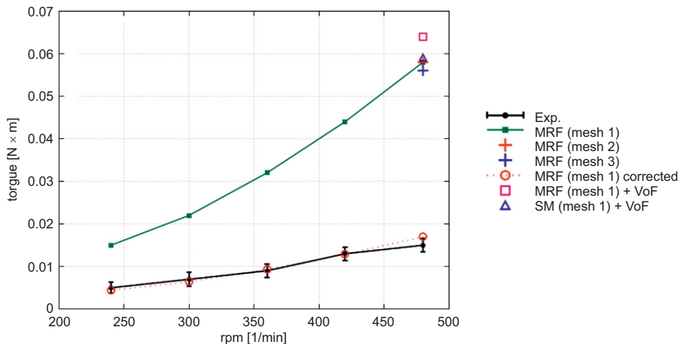
Fig. 14. Torque values as a function of impeller rotational speed
