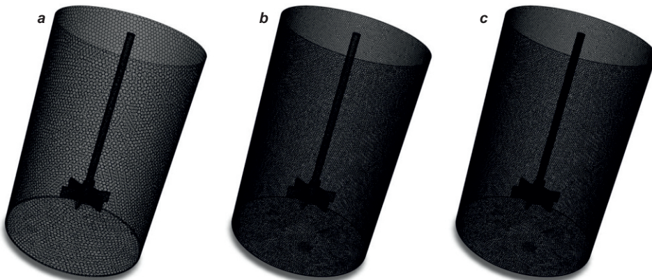
Fig. 6. Polyhedral numerical meshes: a) mesh 1, b) mesh 2, c) mesh 3
