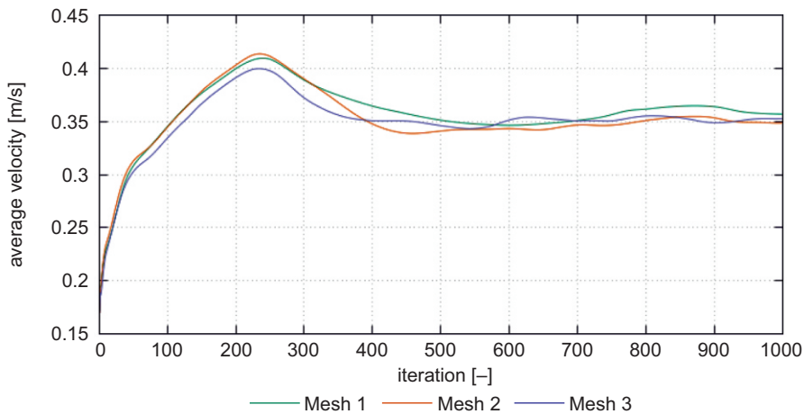
Fig. 9. Average speed monitor graph for the MRF model, 480 rpm, and three mesh variants
