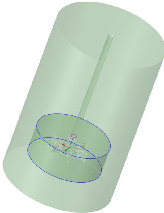
Fig. 4. View of the computational domain divided into a moving and stationary zone
