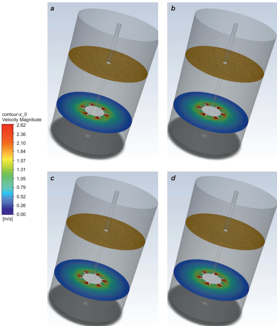
Fig. 13. Visualization of the impeller movement: a) iteration 528, b) iteration 532, c) iteration 536, d) iteration 540
