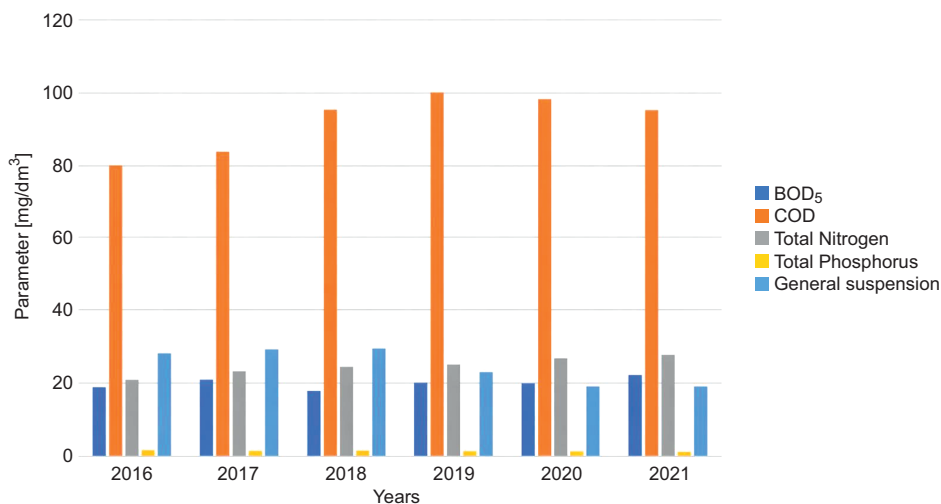
Fig. 2. Comparison of average pollutant values in treated sewage over the years 2016–2021 Source: own work.
