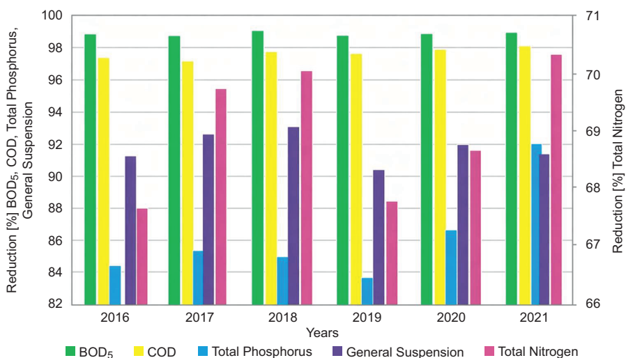
Fig. 3. Pollution reduction rate in 2016–2021 Source: own work.
